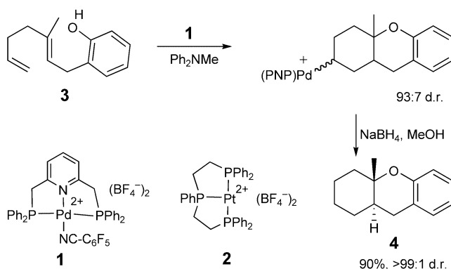
Scheme 1. Phenol trapping of an intermediate cation and reductive cleavage of the stable Pd alkyl complex.
