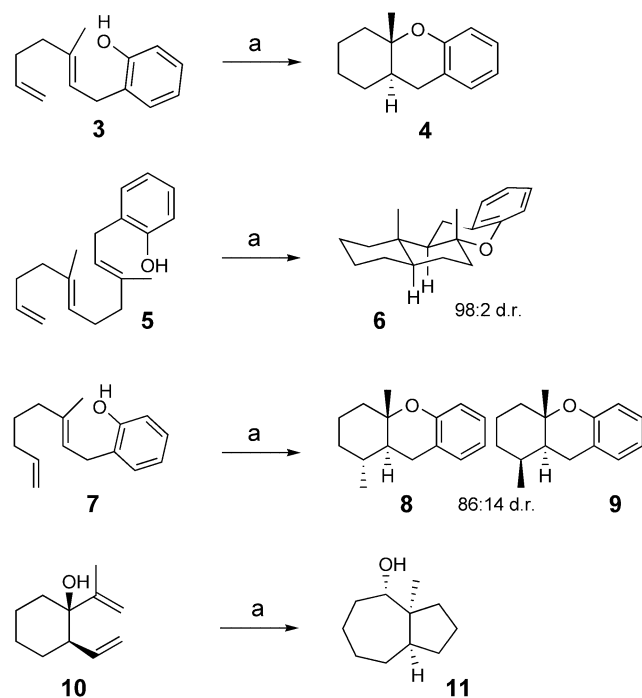
Scheme 2. Interception of cations generated with 2 . Compound 8 was characterized by X-ray crystallography. a: 1) 2 , 1.05 equiv Ph 2 NMe, CH 2 Cl 2 , RT, 1–4 h; 2) NaBH 4 , MeOH.
